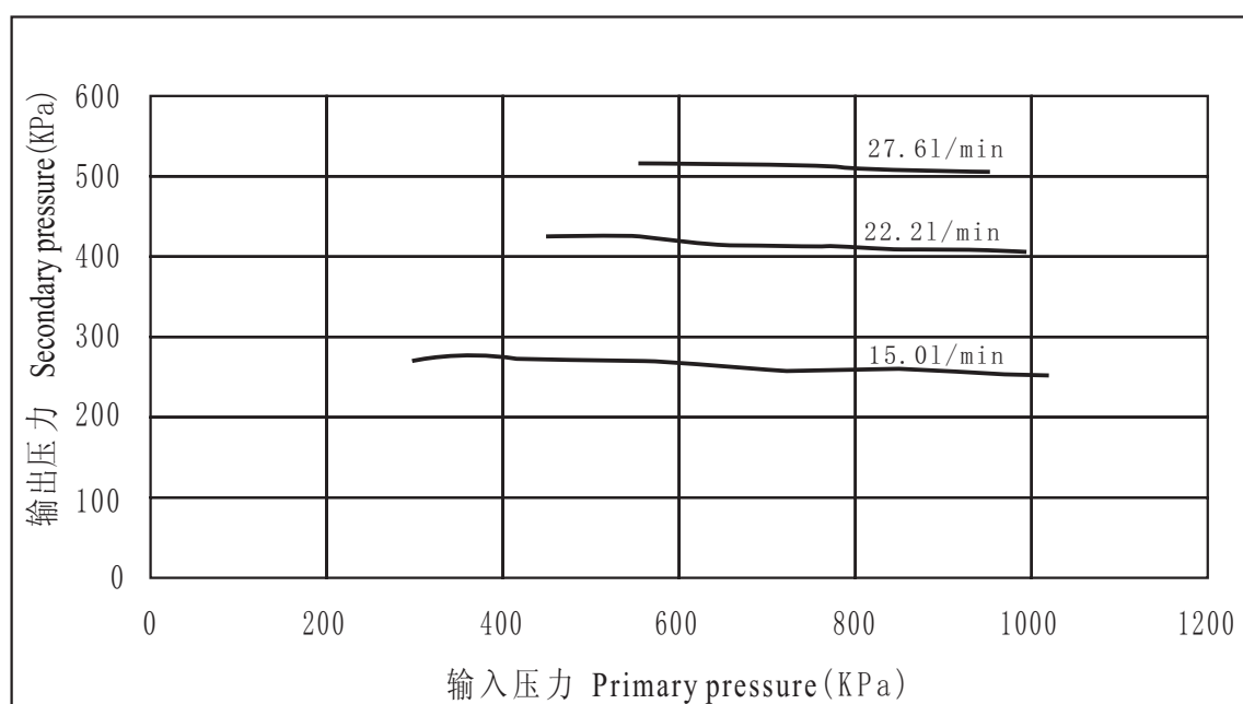
压力调节特性曲线 Pressure characteristics
