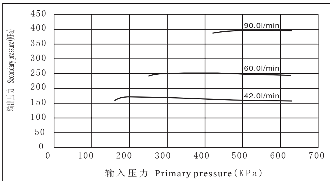
压力调节特性曲线 Pressure characteristics
